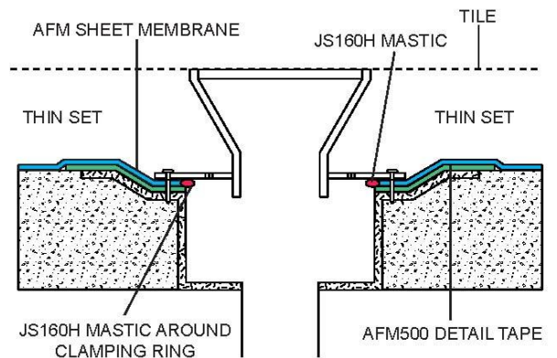
DRAIN DETAIL
